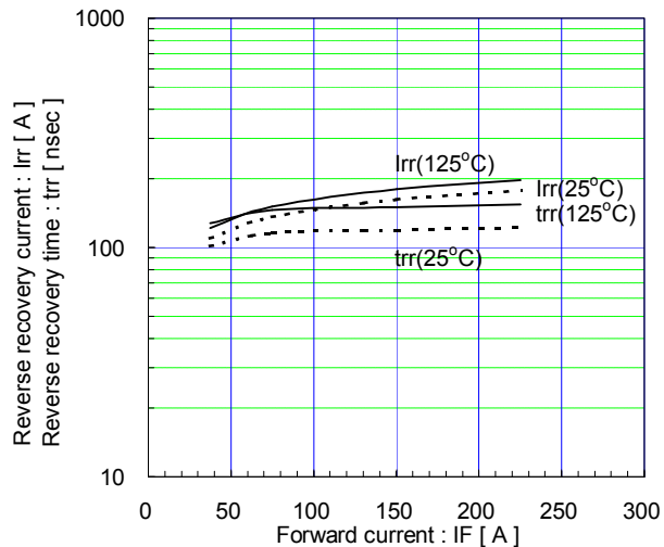
Reverse recovery characteristics (typ.) Vcc=600V, VGE=±15V, RG=4.7Ω
