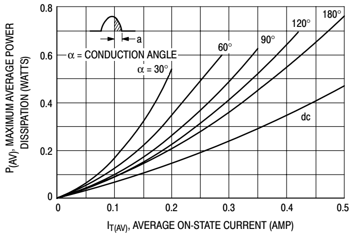
Figure 5. Power Dissipation
