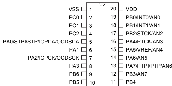
HT66F0181/HT66V0181 20 SOP-A/NSOP-A/SSOP-A
