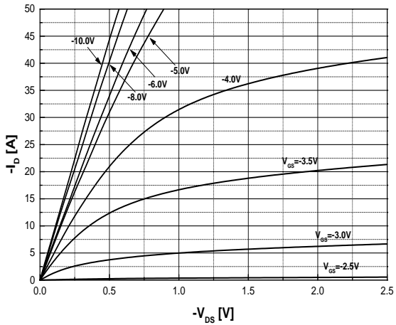
Fig.1 On-Region Characteristics
