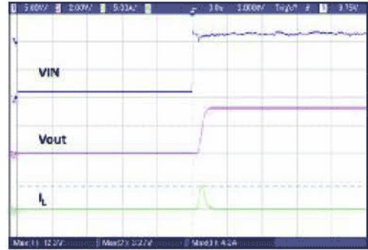
Soft Start & Inrush Current
