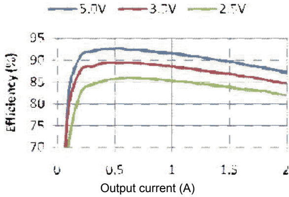
Medium Loading Operation ( I_L=1A )
