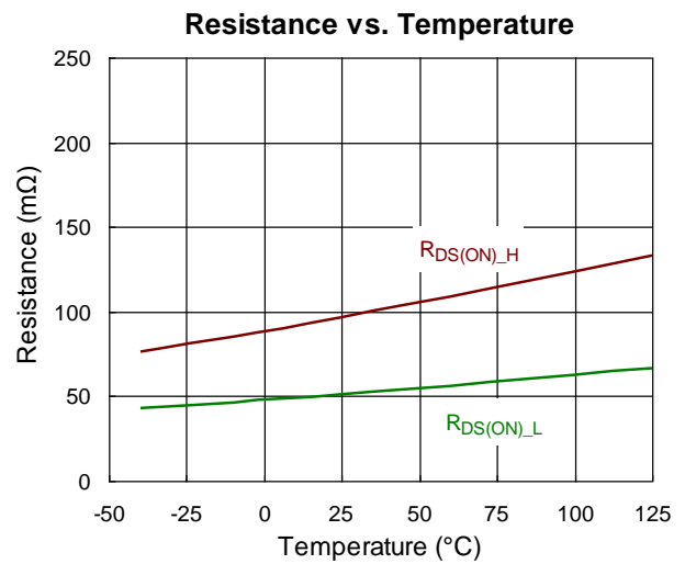
Figure 13. RT6253A/B R_{DS(ON)} vs. Temperature
