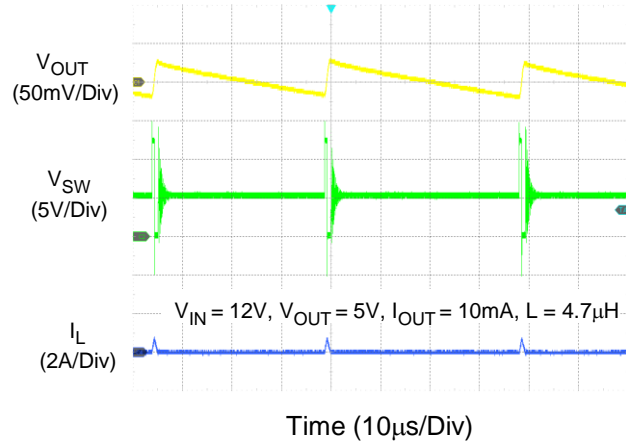
Output Ripple as I_{OUT} = 10mA
