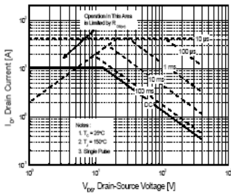
Figure 9-1. Maximum Safe Operating Area for TSP740M
