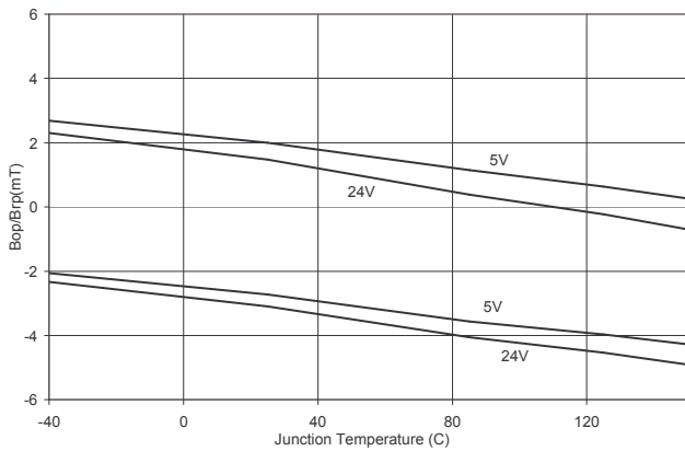
11.3 Magnetic Parameters vs T_J
