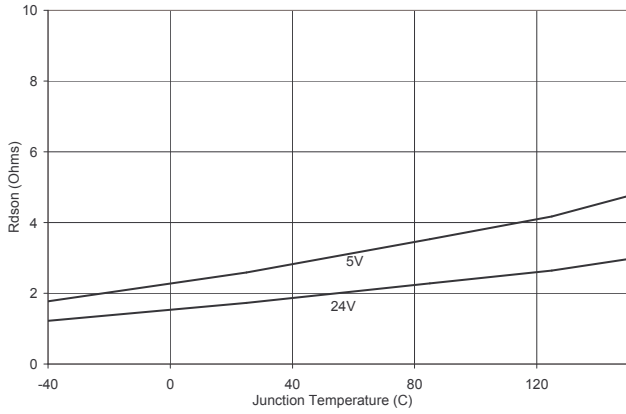
11.1 R_{DS(on)} vs T_J
