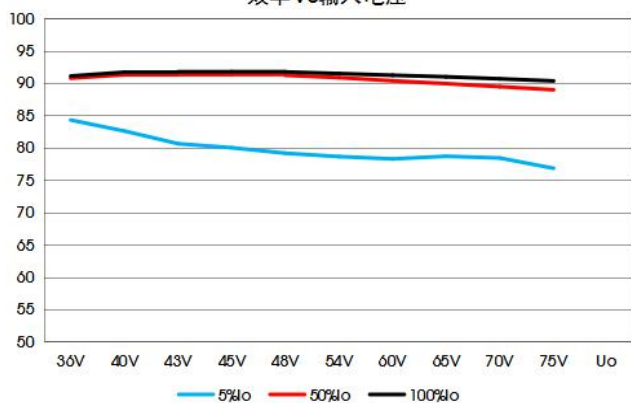
VCF4828EBO-150W(F)R3-N 效率VS输入电压
