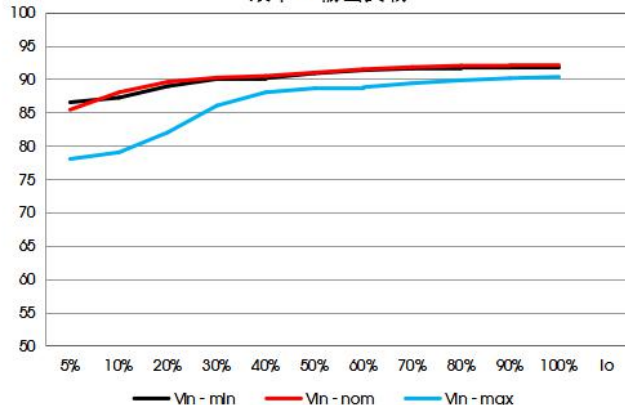
VCF4848EBO-150W(F)R3-N 效率VS输出负载
