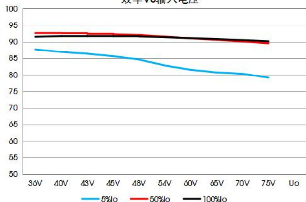
VCF4824EBO-150W(F)R3-N 效率VS输入电压
