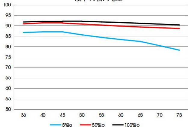
VCF4848EBO-150W(F)R3-N 效率VS输入电压
