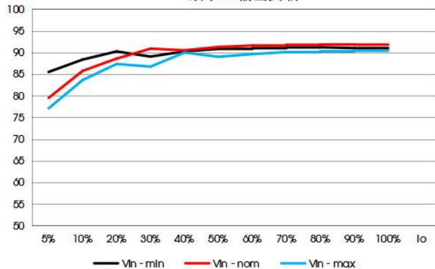
VCF4828EBO-150W(F)R3-N 效率VS输出负载
