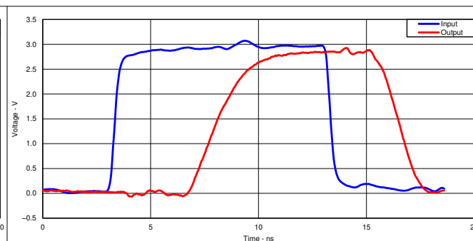
图 7-2. Switching Characteristics at 50 MHz Excellent Signal Integrity (3.3 V to 3.3 V at 3.3-V V_{CC} )
