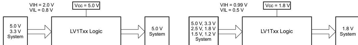
图 9-4. LVxT Up and Down Translation Example
