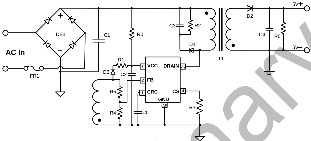
Figure1. Typical Application of PT2313E
